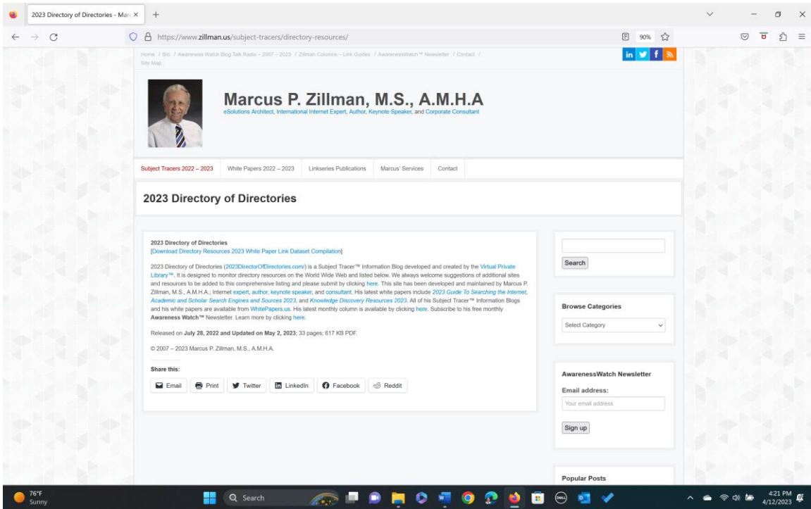
Figure 1: Directory Resources 2023
